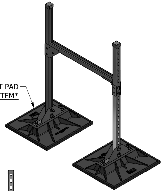
Isometric View
