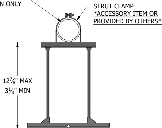
END VIEW
