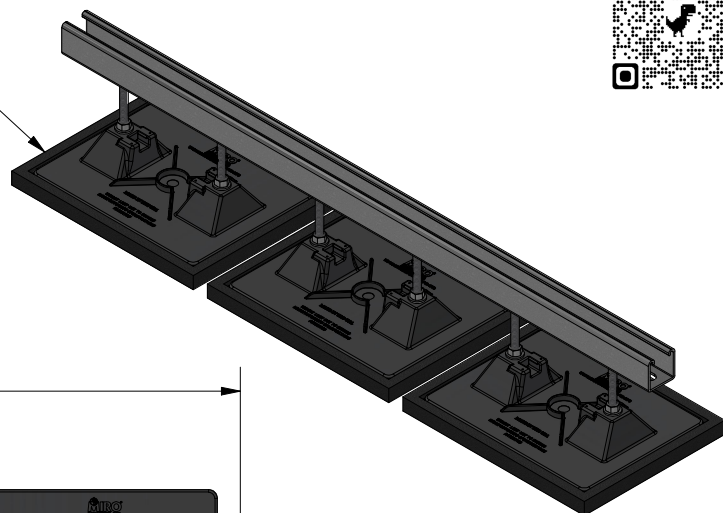
ISOMETRIC VIEW
