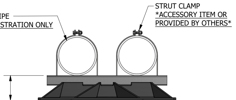
END VIEW
