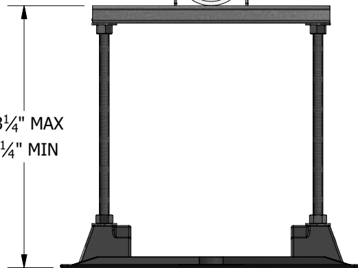
END VIEW
