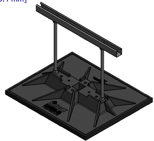
SUPPORT PAD UNDER A MIRO 24-BASE STRUT-18 (NOT INCLUDED)
